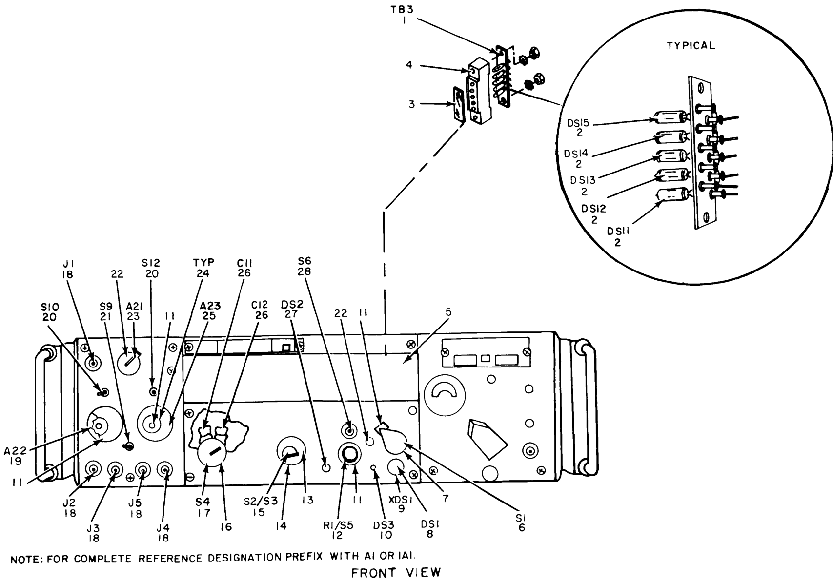
Figure 3. Digital Readouts CP-814/USM-207 and CP-814A/USM-207, Front and Rear Views (Sheet 1 of 2).
