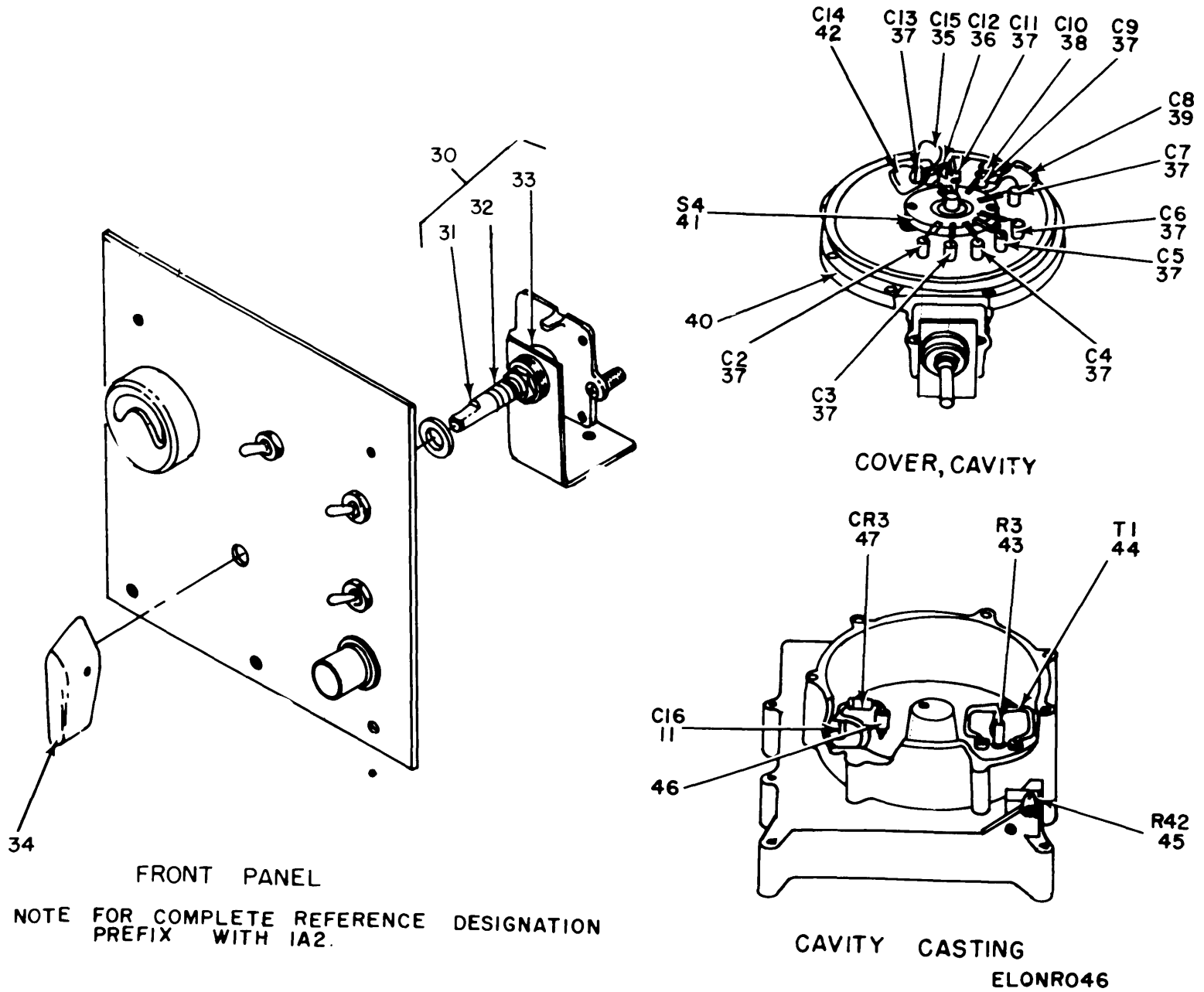
Figure 22. Frequency Converter CV-1921A/USM-207, Serial Numbers 1A thru 1100A (Sheet 2 of 2).
