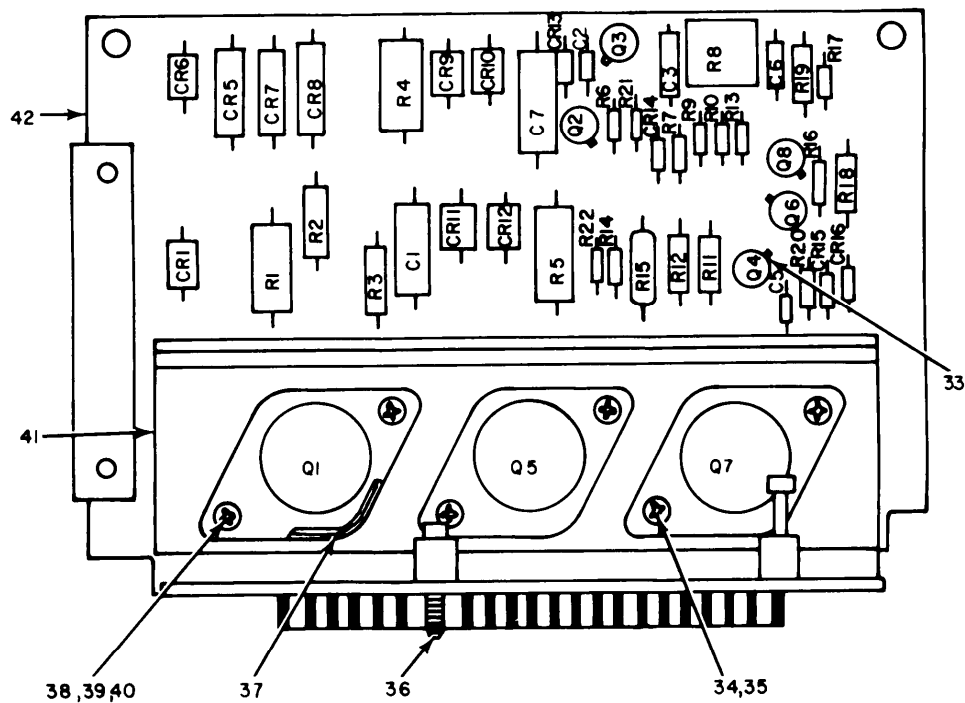
VOLTAGE REGULATOR 5280011-501
