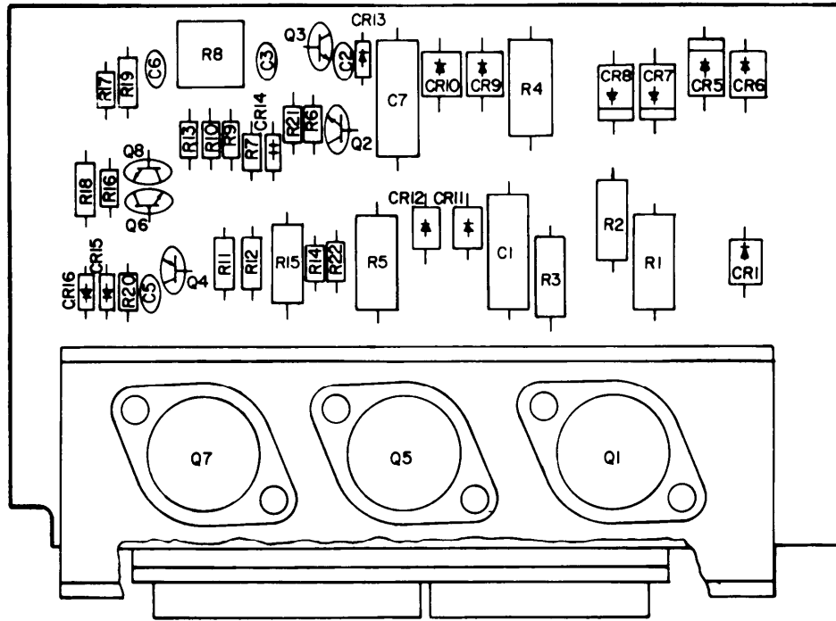
VOLTAGE REGULATOR MP22-524
