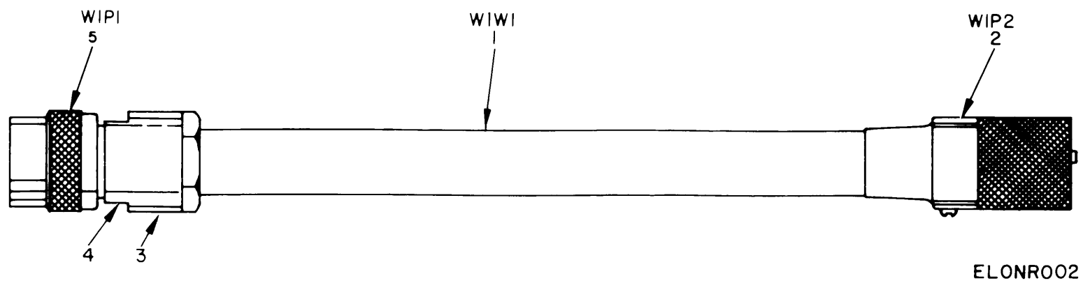
Figure 28. Cable Assembly, Electrical Power (W1).
