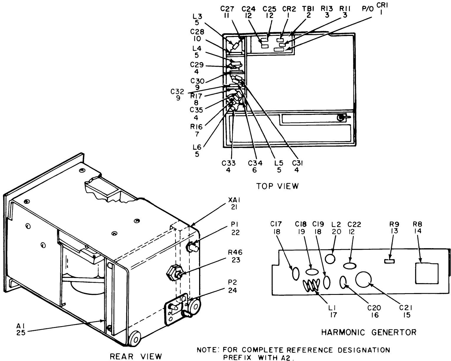
Figure 21. Frequency Converter CV-1921/USM-207, CV-1921A/USM-207 (Sheet 1 of 3).
