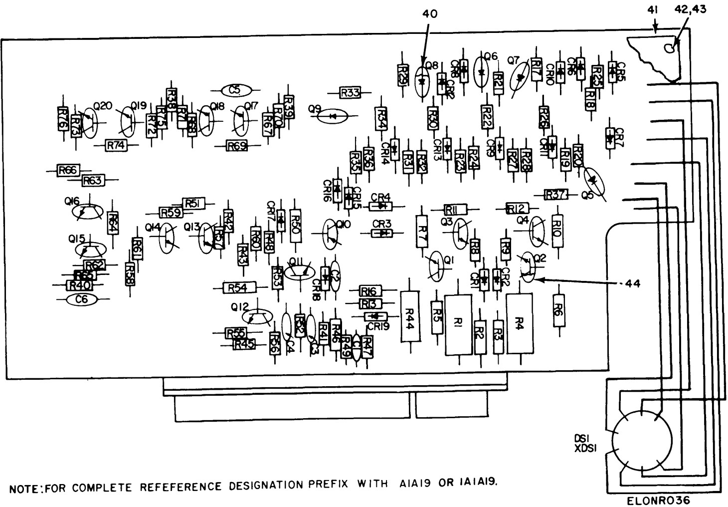
Figure 16. Frequency Divider (A1A19) (Sheet 1 of 2).
