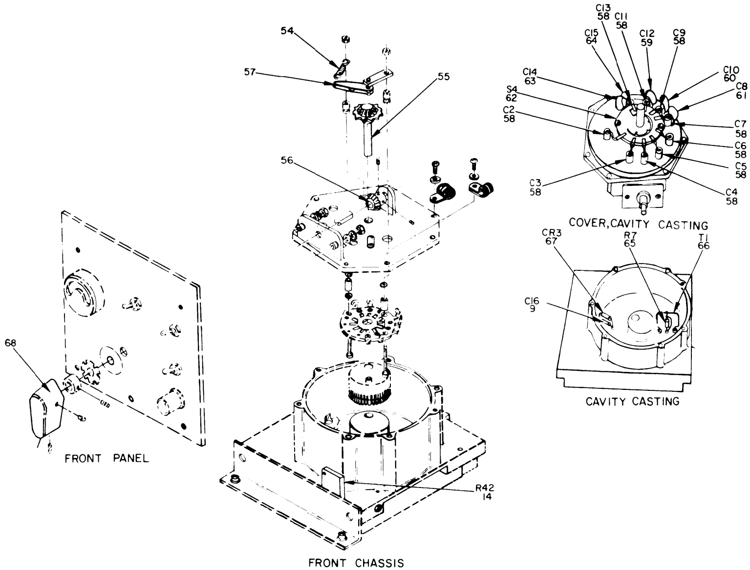
Figure 21. Frequency Converter CV-1921/USM-207, CV-1921A/USM-207 (Sheet 3 of 3).
