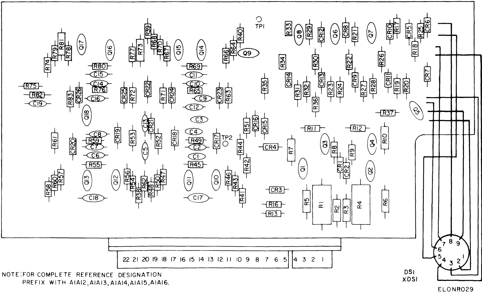
Figure 13. Frequency Dividers (A1A12 Thru A1A16) (Sheet 1 of 2).
