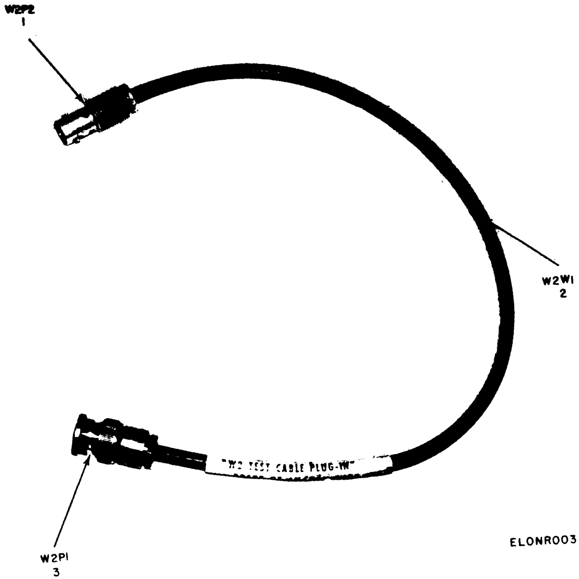
Figure 29. Cable Assembly, Radio Frequency (W2).
